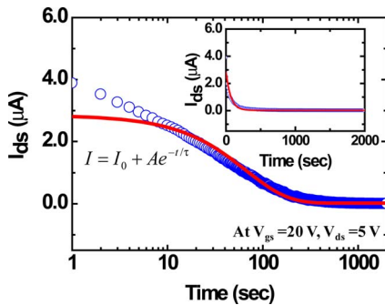
FIG. 2. (Color online) Experimental (circles) and exponential fitting curve (solid line) of drain current decay measured at V_{gs}=20 V and V_{ds}=5 V in ambient air.
