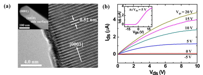
FIG. 1. (Color online) (a) HRTEM image of an individual ZnO nanowire. Inset is the FESEM image of the ZnO nanowire with hexagonal shape. (b) Typical I_{ds} - V_{ds} curves at different gate biases from -5 to 20 V, with 5 V steps. Inset is I_{ds} - V_{gs} curve measured at V_{ds}=5 V.
