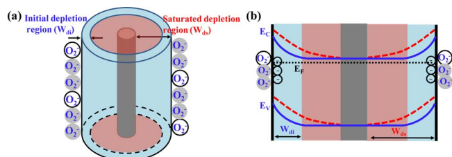
FIG. 4. (Color online) (a) Schematic diagram and (b) energy band diagram explaining the initial depletion region ( W_{di} ) and saturated depletion region ( W_{ds} ) of ZnO nanowire FET due to oxygen trapping at a prolonged positive gate bias. E_C , E_F , and E_V are the conduction band, the Fermi energy level, and the valence band, respectively.
